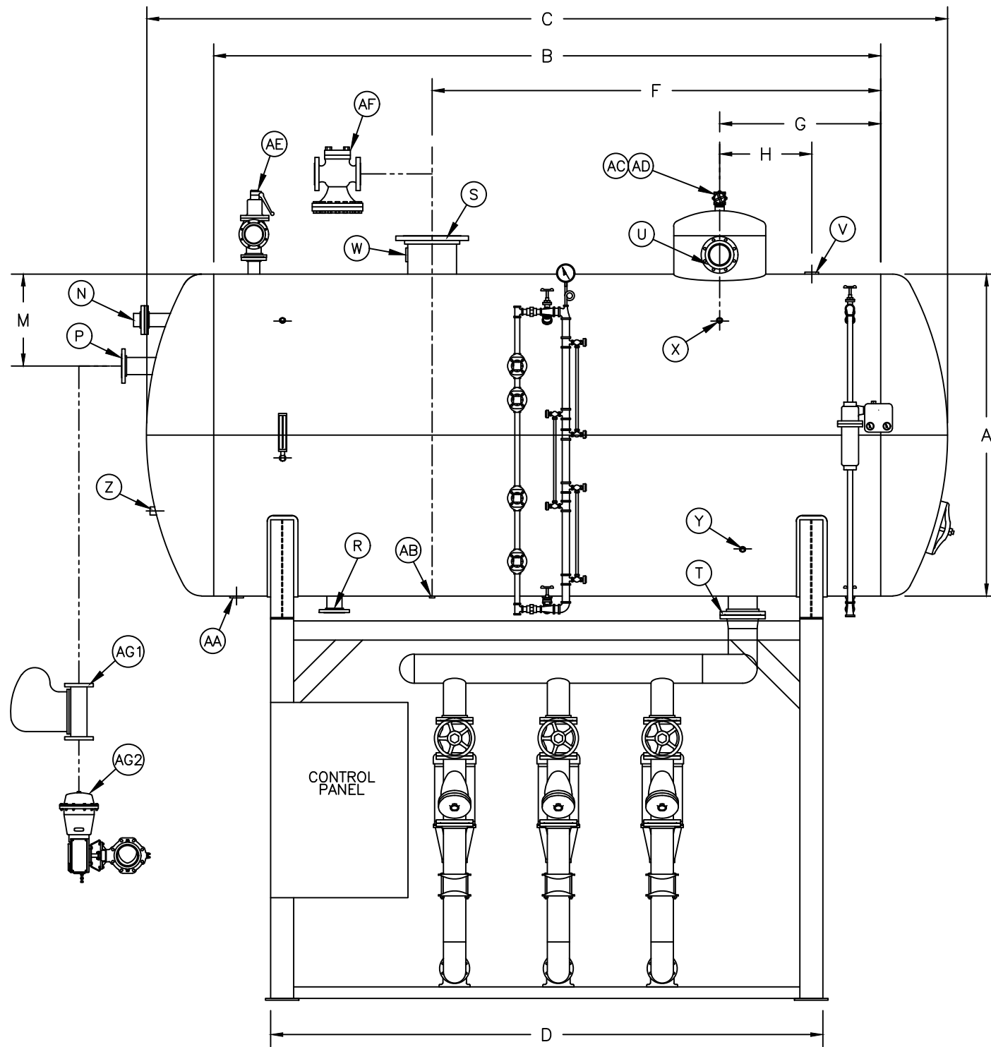
FRONT VIEW UNITS 150MS THRU 500MS
